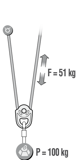
6B. 2:1 hauling system
