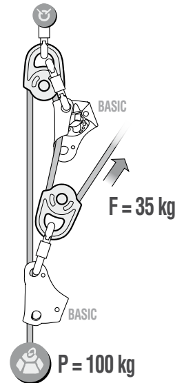
6C. 3:1 hauling system with progress capture
